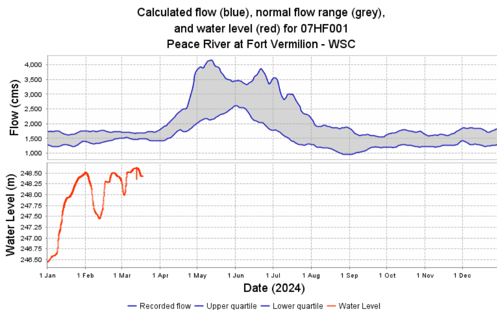
Figure 33. Calculated and normal flow range for Lower Peace River basin at Fort Vermillion, Alberta, retrieved March 17, 2024 from AEPA.
