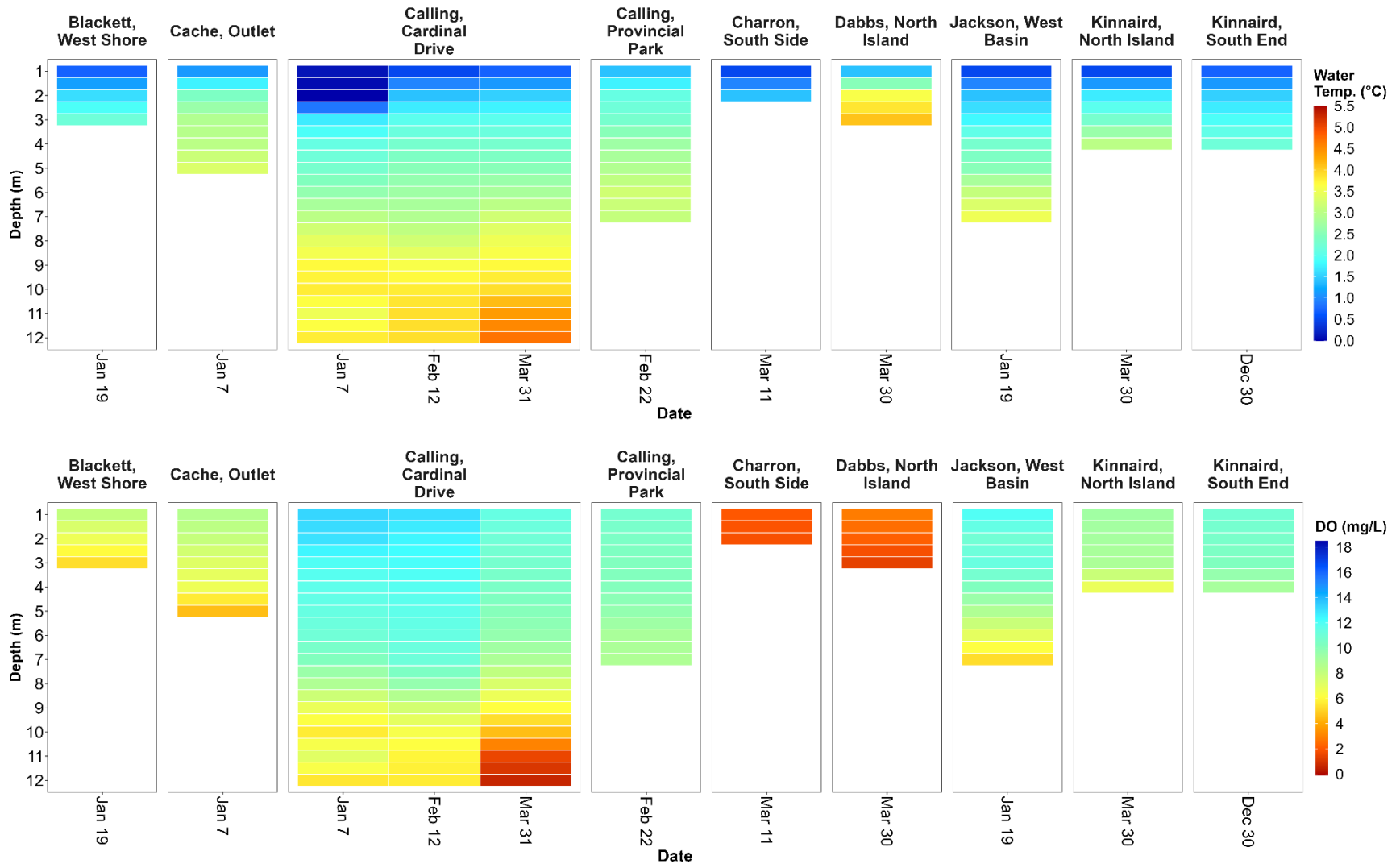
Figure 16a. Water temperature (Water Temp.; °C) and dissolved oxygen (DO; mg/L) measurements recorded at lakes sampled in the Athabasca River watershed in the Winter LakeKeepers 2022-2023 season. Measurements were taken at 0.1m and 0.5m, then every meter starting at 1 meter from ice surface, until lake bottom, however only measurements at 1m and below are plotted. Note that the measurements are linearly interpolated to 0.5m increments to improve data visualization.
