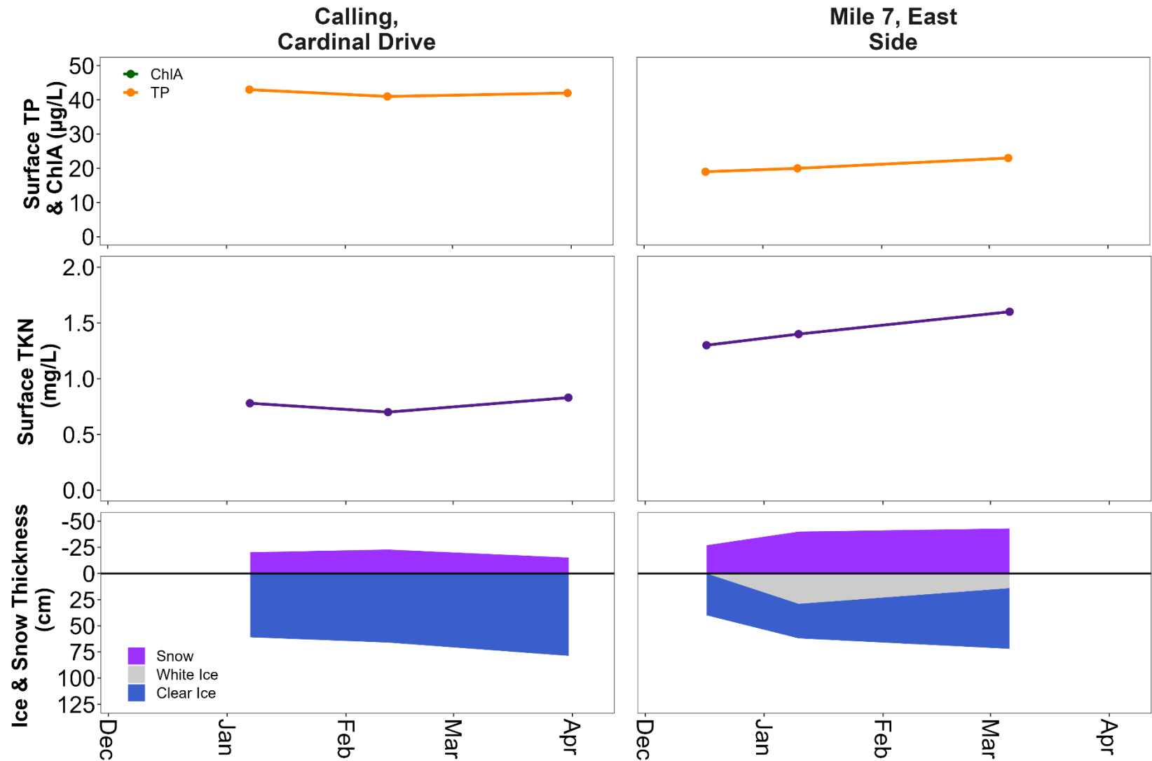
Figure 17. Seasonal surface water chemistry (TP = total phosphorus and ChIA = chlorophyll-a, Top; TKN = total Kjeldahl nitrogen, middle) and ice (clear and white) and snow thickness (bottom) from lakes sampled in the Athabasca River watershed in the Winter LakeKeepers 2022 season. In the top panel, TP is orange and ChIA is green, TKN in the middle section is purple, and in the bottom section snow is pink, white ice is gray, and clear ice is blue. Note that ice and snow thickness is plotted in reference to the ice surface (horizontal black line).
