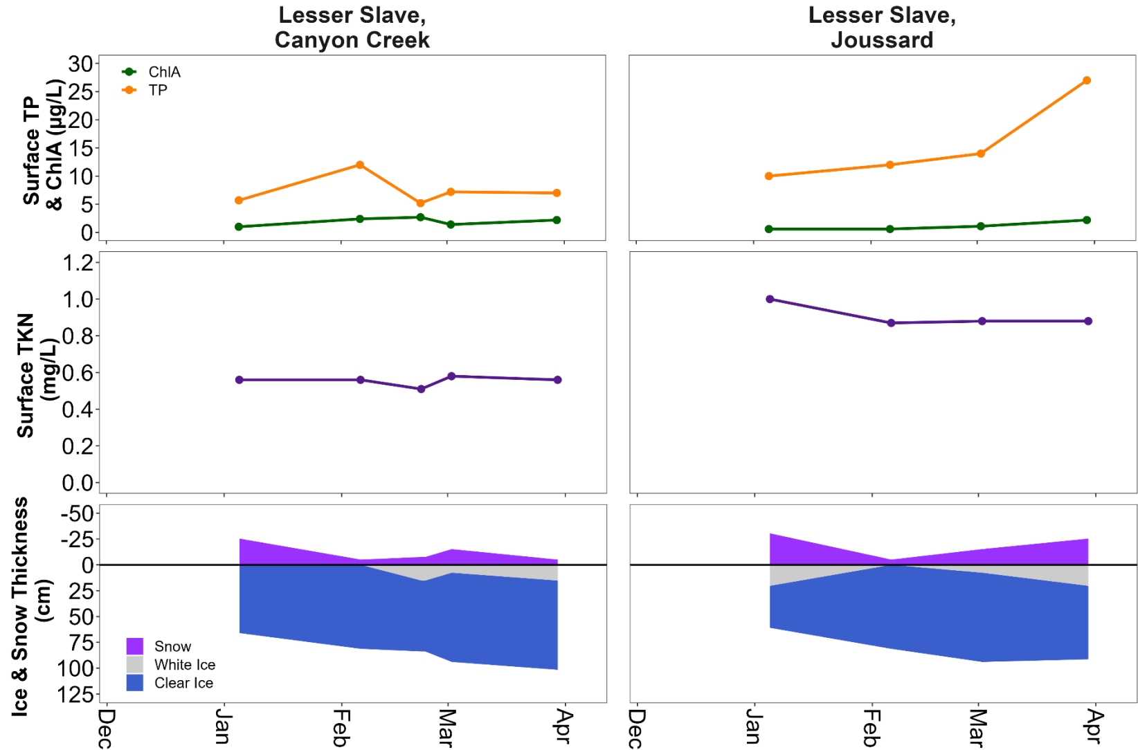
Figure 19. Seasonal surface water chemistry (TP = total phosphorus and ChlA = chlorophyll-a, Top; TKN = total Kjeldahl nitrogen, middle) and ice (clear and white) and snow thickness (bottom) from lakes sampled in the Lesser Slave Lake watershed in the Winter LakeKeepers 2022 season. In the top panel, TP is orange and ChlA is green, TKN in the middle section is purple, and in the bottom section snow is pink, white ice is gray, and clear ice is blue. Note that ice and snow thickness is plotted in reference to the ice surface (horizontal black line).
