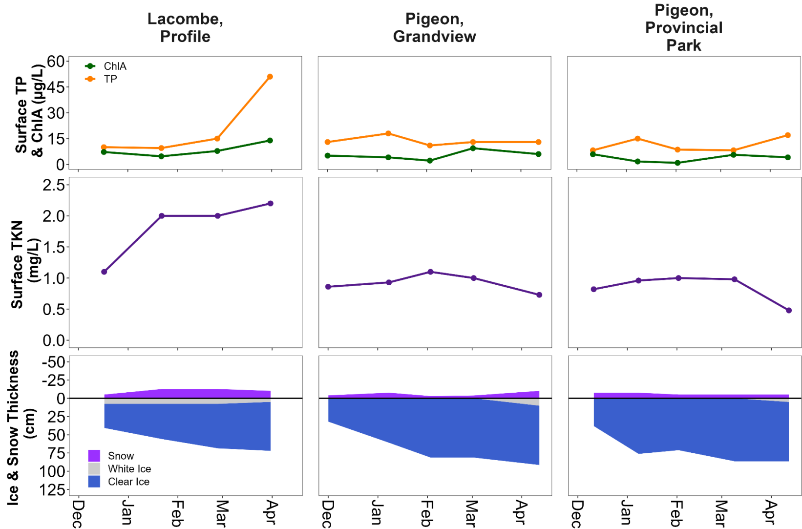
Figure 25. Seasonal surface water chemistry (TP = total phosphorus and ChlA = chlorophyll-a, Top; TKN = total Kjeldahl nitrogen, middle) and ice (clear and white) and snow thickness (bottom) from lakes sampled in the Battle River watershed in the Winter LakeKeepers 2022 season. In the top panel, TP is orange and ChlA is green, TKN in the middle section is purple, and in the bottom section snow is pink, white ice is gray, and clear ice is blue. Note that ice and snow thickness is plotted in reference to the ice surface (horizontal black line).
