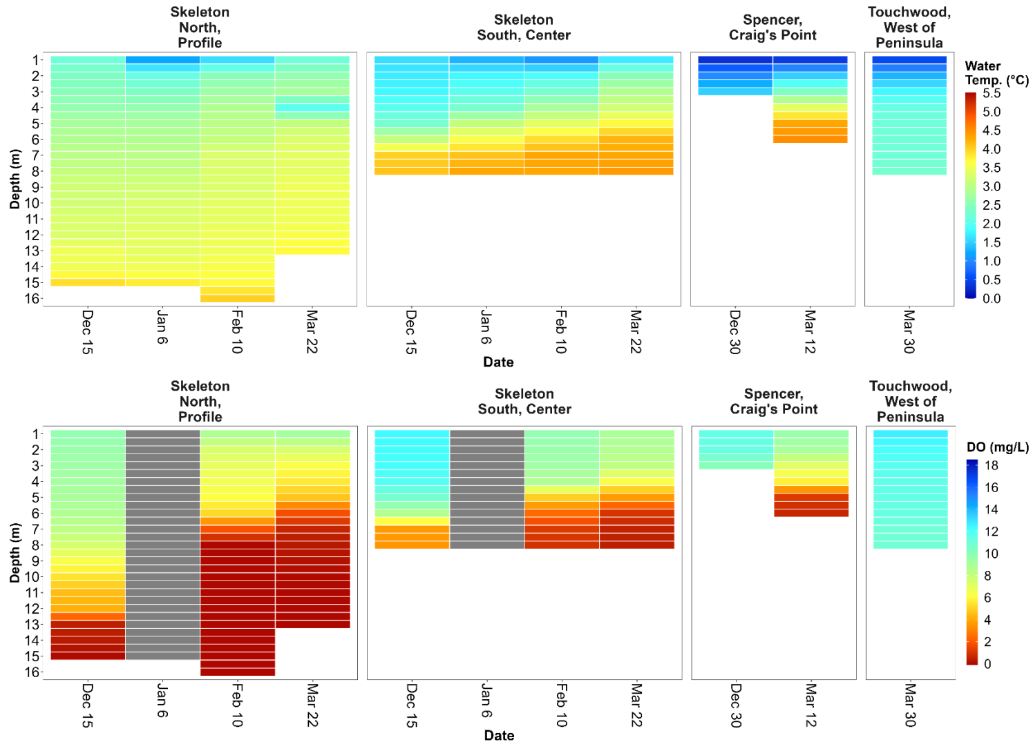
Figure 20b. Water temperature (Water Temp.; °C) and dissolved oxygen (DO; mg/L) measurements recorded at lakes sampled in the Beaver River watershed in the Winter LakeKeepers 2022-2023 season. Measurements were taken at 0.1m and 0.5m, then every meter starting at 1 meter from ice surface, until lake bottom, however only measurements at 1m and below are plotted. Note that the measurements are linearly interpolated to 0.5m increments to improve data visualization. Note that DO measurements from 'Skeleton North, Profile' and 'Skeleton South, Center' taken on January 6 th , 2023 are unavailable.
