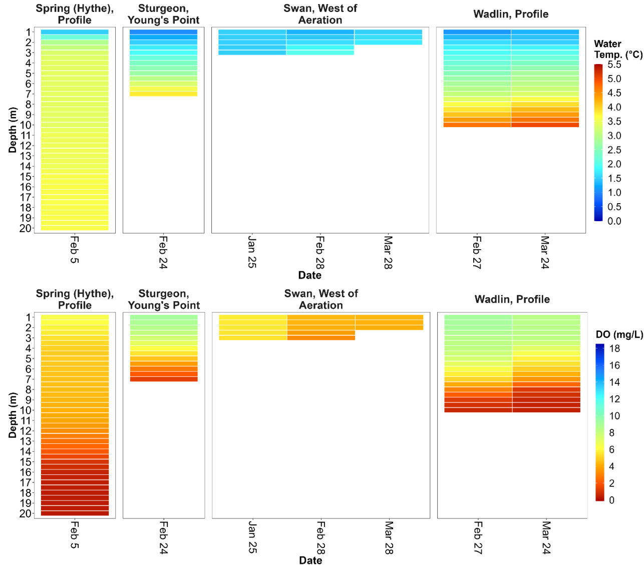
Figure 14. Water temperature (Water Temp.; °C) and dissolved oxygen (DO; mg/L) measurements recorded at lakes sampled in the Peace River watershed in the Winter LakeKeepers 2022-2023 season. Measurements were taken at 0.1m and 0.5m, then every meter starting at 1 meter from ice surface, until lake bottom, however only measurements at 1m and below are plotted. Note that the measurements are linearly interpolated to 0.5m increments to improve data visualization.
