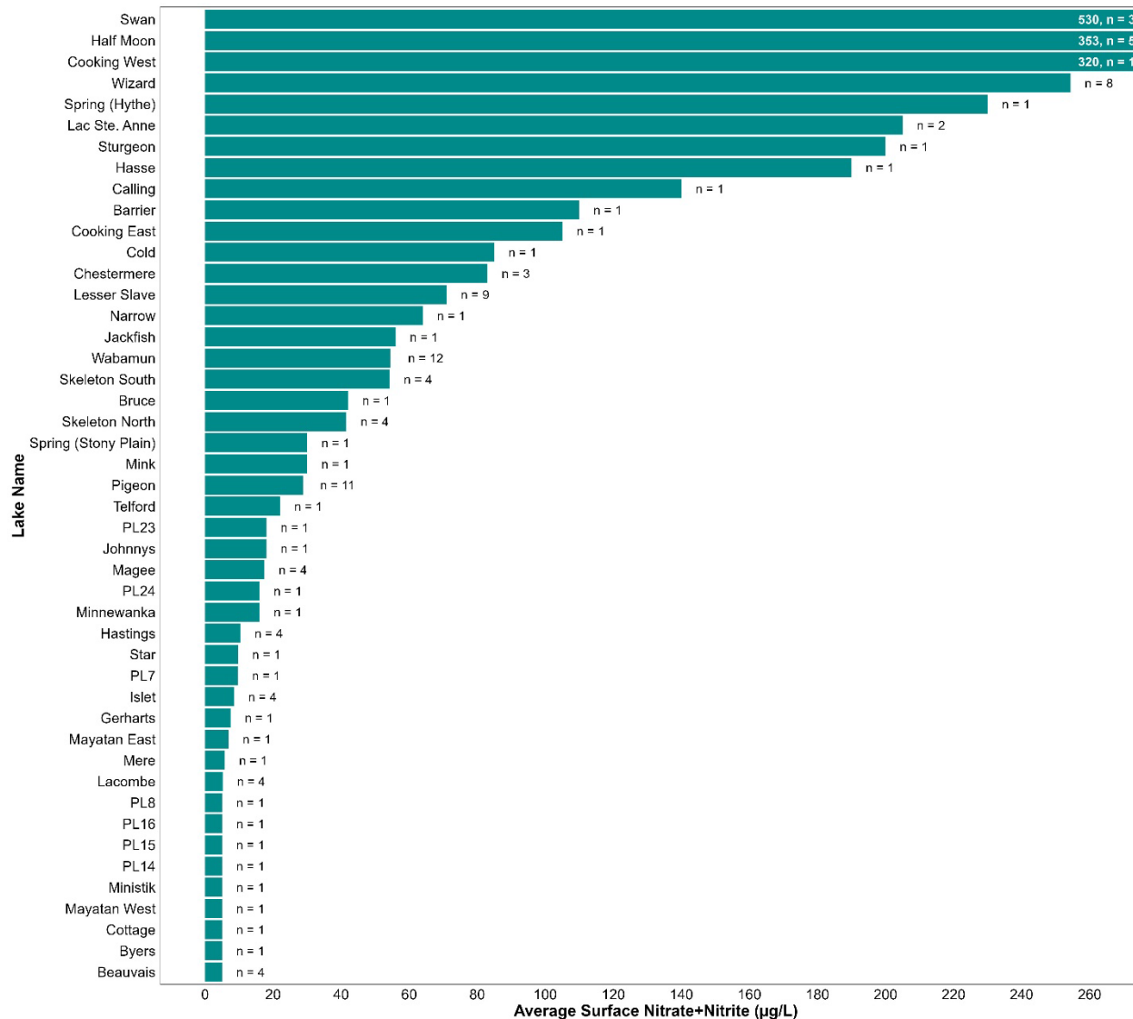
Figure 6. Average sum of surface nitrate and nitrite (µg/L) from lakes sampled in the Winter LakeKeepers 2022-2023 season. Average sum of surface nitrate and nitrite represents the average from across sample dates, if lakes had multiple sample events, and across sample locations, if lakes had multiple sampled locations (number of samples indicated by the "n" value beside each bar). Samples were taken at 0.5m at the sampling location, between November 2022 and April 2023. Extreme outliers on the upper range (>3*IQR) are not fully plotted.
