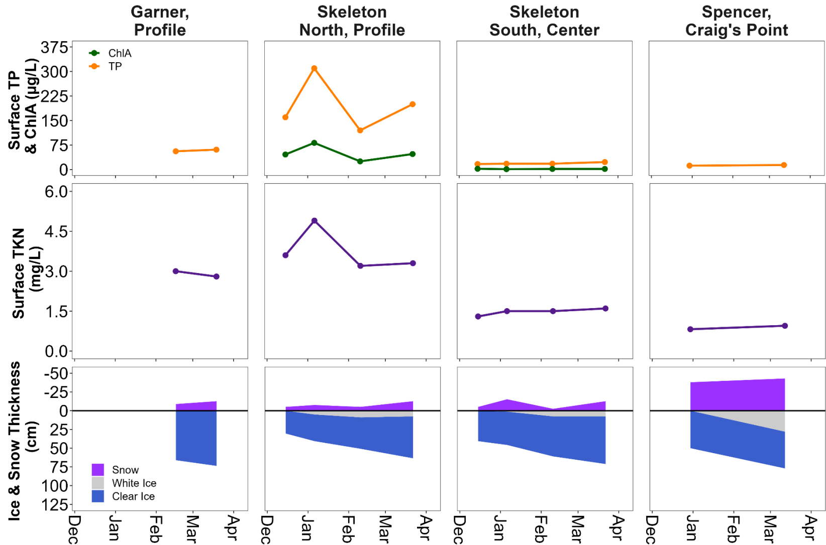
Figure 21. Seasonal surface water chemistry (TP = total phosphorus and ChlA = chlorophyll-a, Top; TKN = total Kjeldahl nitrogen, middle) and ice (clear and white) and snow thickness (bottom) from lakes sampled in the Beaver River watershed in the Winter LakeKeepers 2022 season. In the top panel, TP is orange and ChlA is green, TKN in the middle section is purple, and in the bottom section snow is pink, white ice is gray, and clear ice is blue. Note that ice and snow thickness is plotted in reference to the ice surface (horizontal black line).
