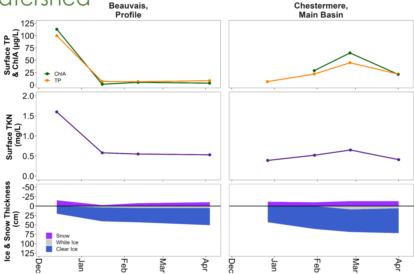
Figure 29. Seasonal surface water chemistry (TP = total phosphorus and ChlA = chlorophyll-a, Top; TKN = total Kjeldahl nitrogen, middle) and ice (clear and white) and snow thickness (bottom) from lakes sampled in the Bow River and Oldman watersheds in the Winter LakeKeepers 2022 season. In the top panel, TP is orange and ChlA is green, TKN in the middle section is purple, and in the bottom section snow is pick, white ice is gray, and clear ice is blue. Note that ice and snow thickness is plotted in reference to the ice surface (horizontal black line).
