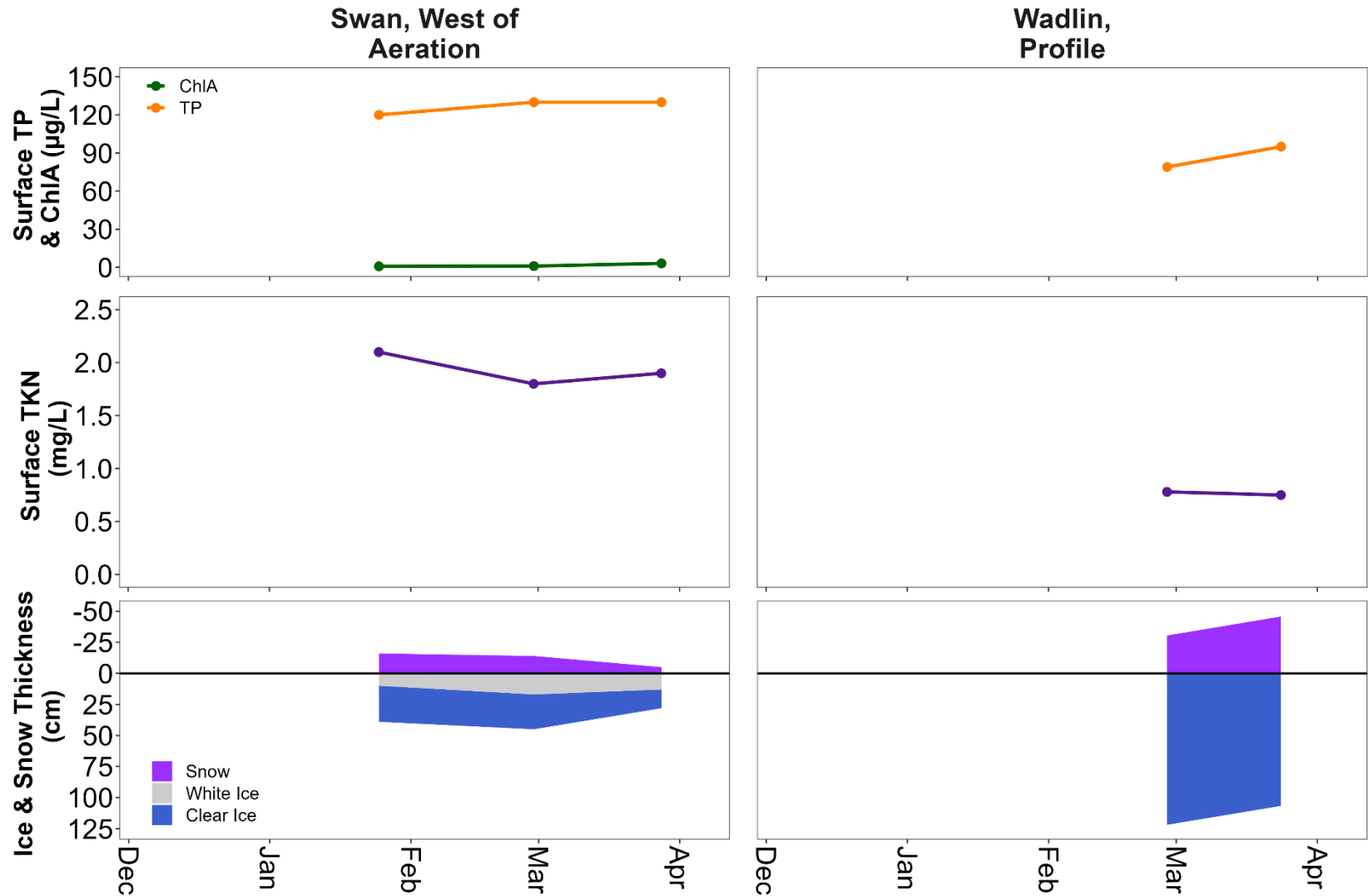
Figure 15. Seasonal surface water chemistry (TP = total phosphorus and ChlA = chlorophyll-a, Top; TKN = total Kjeldahl nitrogen, middle) and ice (clear and white) and snow thickness (bottom) from lakes sampled in the Peace River watershed in the Winter LakeKeepers 2022 season. In the top panel, TP is orange and ChlA is green, TKN in the middle section is purple, and in the bottom section snow is pink, white ice is gray, and clear ice is blue. Note that ice and snow thickness is plotted in reference to the ice surface (horizontal black line).
